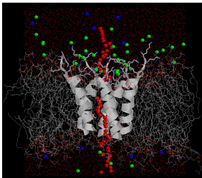
Fig. 1. Initial conformations of umbrella sampling simulations. The pentameric p22 pore is represented using cartoon, with the oligo-lysine C-terminal tail shown in sticks. The POPC lipids are shown in thin sticks and only the oxygen atoms of water molecules are shown as red dots. \text{Cl}^- and \text{K}^+ ions are shown as green and blue spheres, respectively. The initial placements of a selected \text{Cl}^- for all 61 umbrella-sampling windows are overlaid on the initial conformation for the z = -30 Å window and then shown as red spheres.
