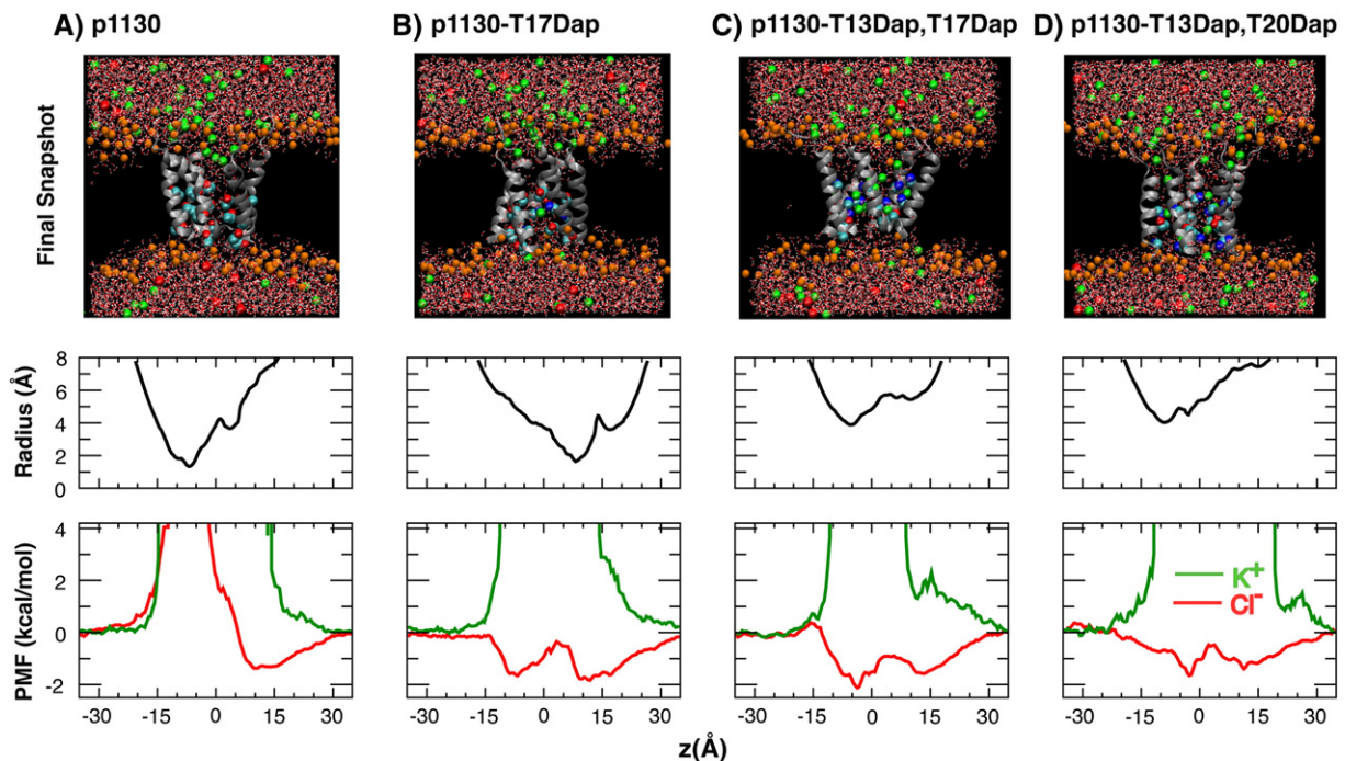
Fig. 6. Summary of equilibrium simulations of p1130 and several singly and doubly Dap substituted sequences. The pore profiles (middle row) were computed using HOLE based on the last snapshots shown (top row). The PMFs (bottom row) were converted directly from the equilibrium ion densities. Note that regions with high free energies (e.g., >3 kcal/mol) are not converged in equilibrium simulations. The lipid molecules are not shown in the snapshots for clarity. Green spheres represent Cl^- ions and yellow spheres represent phosphorus atoms of lipid head groups.
