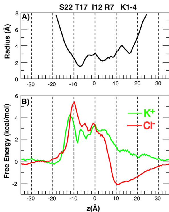
Fig. 4. The pore radius and overall PMFs of \text{K}^+ and \text{Cl}^- permeation through the model p22 pentameric pore. Approximate locations of several key residues are marked. The overall PMFs were constructed by combining the results from umbrella sampling and equilibrium simulations using linear interpolation (see Materials and methods). The pore radius profile was computed using HOLE [47].
