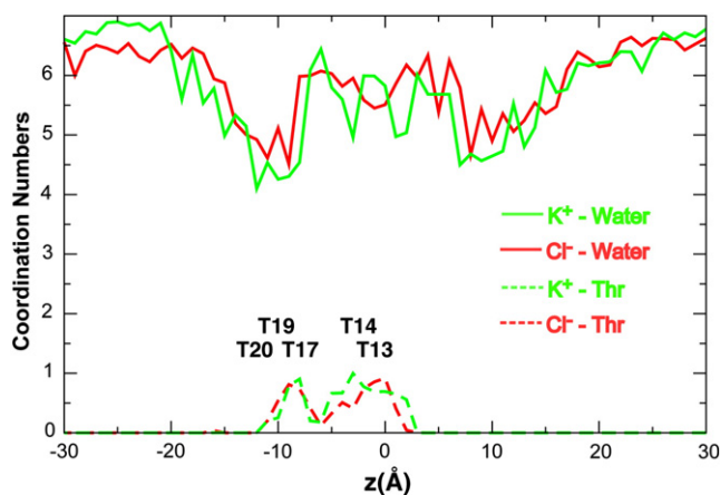
Fig. 5. Average numbers of coordinating water molecules and threonine hydroxyls as a function of z displacement from the pore center of mass. The approximate locations of rings of threonine hydroxyls are also marked.
