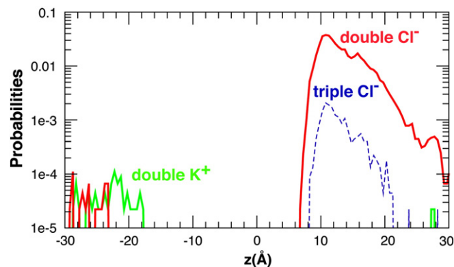
Fig. 3. Probabilities of finding multiple ions within the 8 Å-radius cylinder centered at the pore center of mass as a function of the z displacement. These probabilities were derived from the 20-ns equilibrium simulation trajectory [28]. Two or more ions were considered to be occupying the same xy -plane if their separation along z -axis was no bigger than 0.5 Å. The probabilities of more than double K^+ or triple Cl^- occupancy were small and thus not shown.
