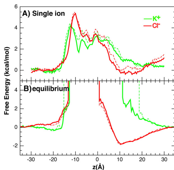
Fig. 2. Free energy profiles as calculated from A) umbrella sampling and B) equilibrium simulations. The thick lines were computed using all data (1 ns per window in umbrella sampling and 20 ns in equilibrium simulation), and the thin dashed lines were computed using only the second half of the data. The equilibrium free energy profiles were converted from the probability distributions of finding either K^+ or Cl^- within the 8 Å-radius cylinder centered at the center of mass of the pore. z is the displacement from the center of the mass of the pore along the membrane normal.
